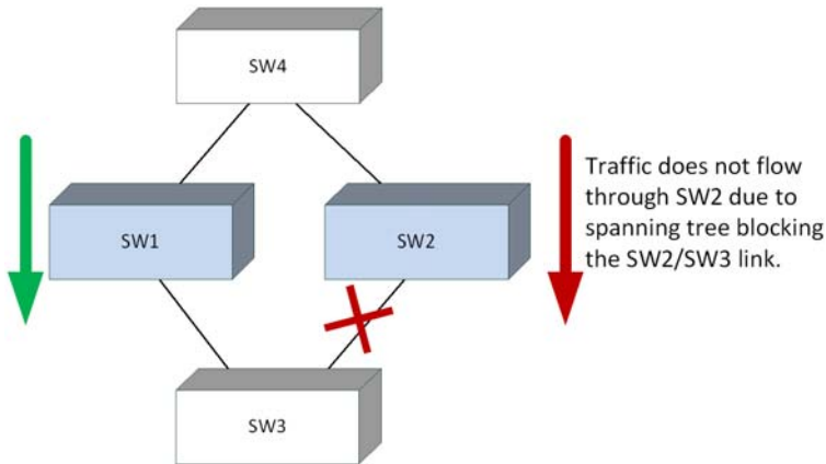
Figure 26-8. STP Blocking
