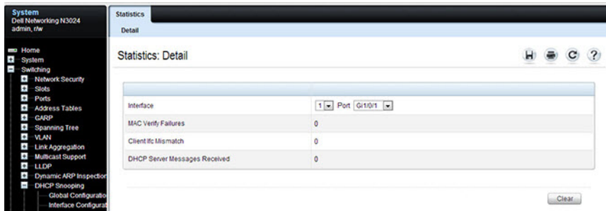
Figure 25-11. DHCP Snooping Statistics
