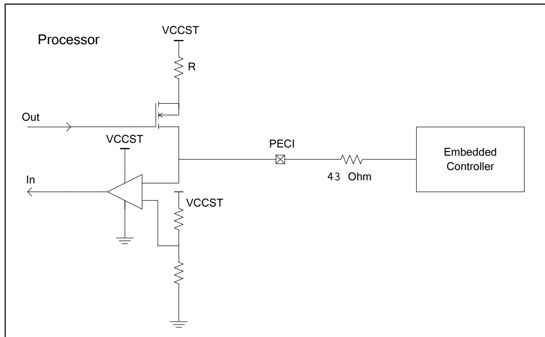
Figure 2-10. Example for PECE EC Connection
