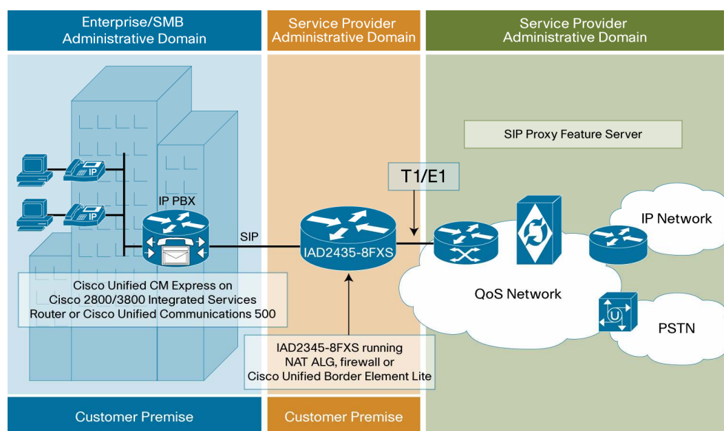
Figure 3. Managed SIP Trunking for IP/PBX Interconnections
