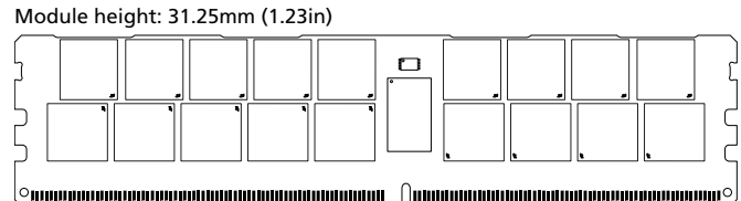
Figure 2: 288-Pin LRDIMM (MO-309, R/C-E2)
