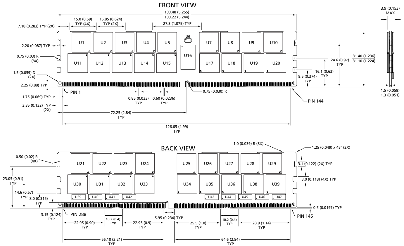
Figure 5: 288-Pin DDR4 LRDIMM
