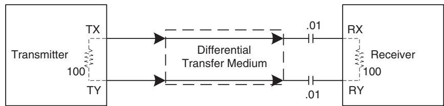
Figure 11. SAS transmitters and receivers
