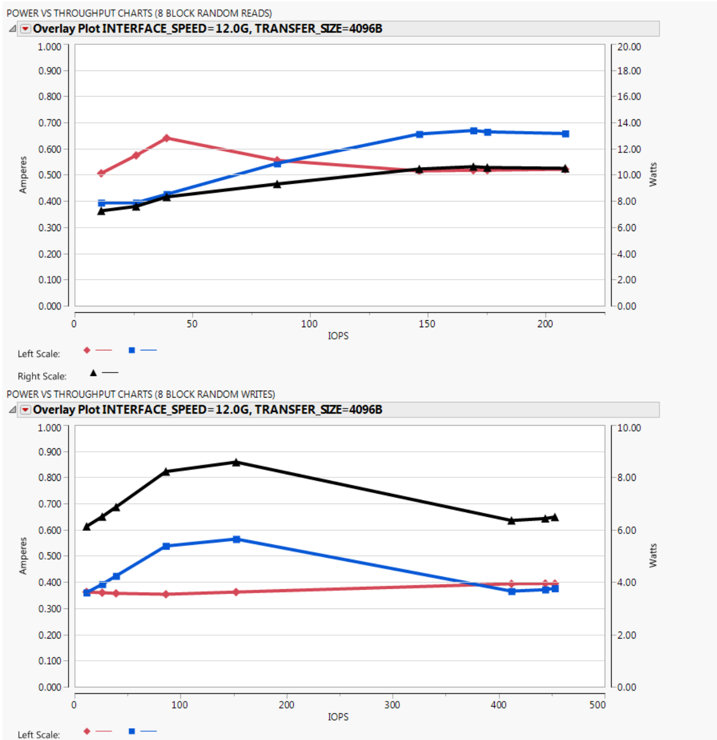
Figure 2. 12TB models (12Gb) DC current and power vs. input/output operations per second
