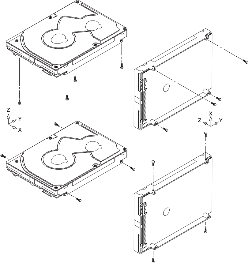
Figure 4. Recommended mounting
